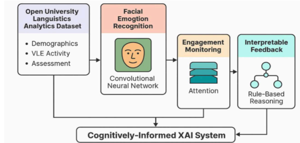
Figure 1 Cognitively-Informed Explainable AI Framework for Education: Integrating Emotion Recognition, Cognitive Reasoning, and Transparent Engagement Monitoring
