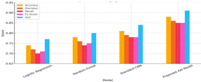
Figure 10 The benchmark comparison of engagement prediction models
