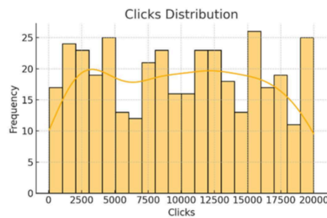
Figure 6 Clicks Distribution
