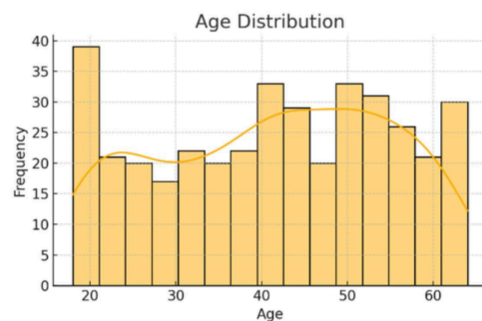
Figure 4 Age Distribution
